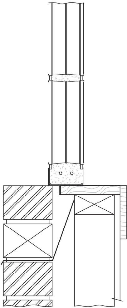
SILL
