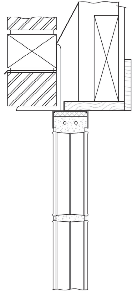
HEAD
